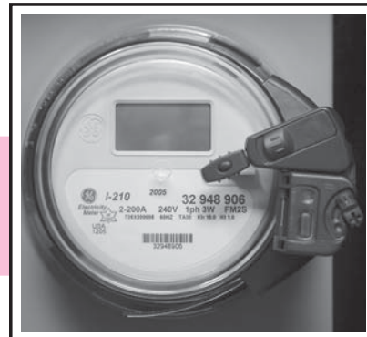
Electronic Meter Front Optical Port AT LEAST 1½ inches from outer rim of dome. If in doubt, physically measure the distance.
